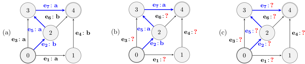
Figure 3: Information revealed in different settings: (a) full information (b) semi-bandit (c) full bandit. The name of each transition e and its output symbol (if revealed) are shown next to it separated by a ‘:’. The blue path indicates the path expert predicted by the learner at round t .
